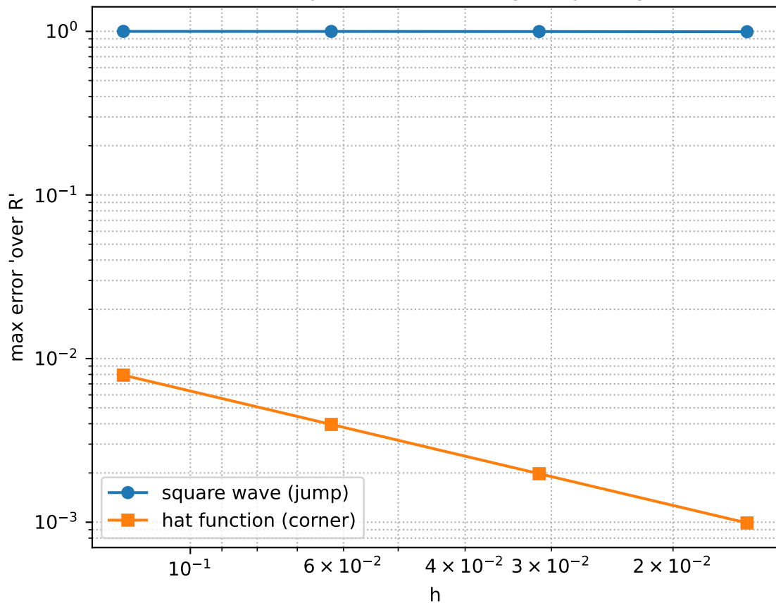
Sinc-interpolation error vs. grid spacing h
